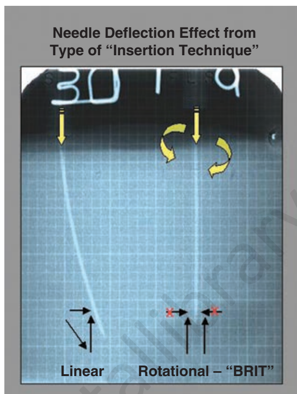
Figure 6-7. BRIT (bi-rotational insertion technique).
