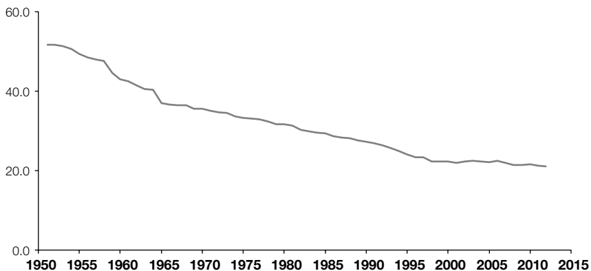
Average span of public listing for companies active in a given year
